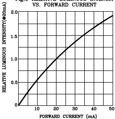
Fig.5 RELATIVE LUMINOUS INTENSITY VS. FORWARD CURRENT
